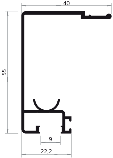
AF - 49AL Trilho Superior 6,10mm
